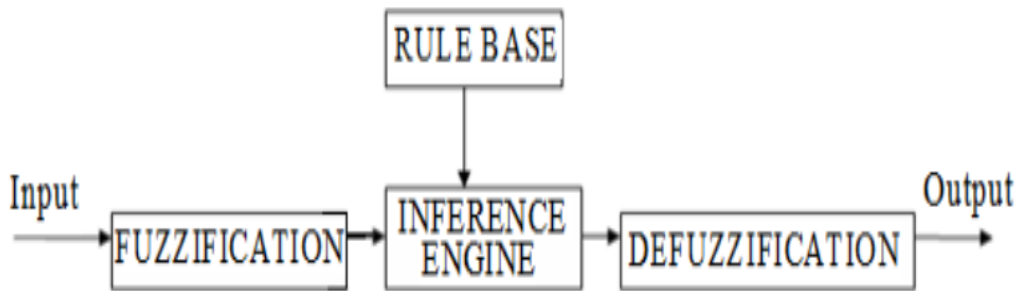
Fig 4: Components of a fuzzy controller
