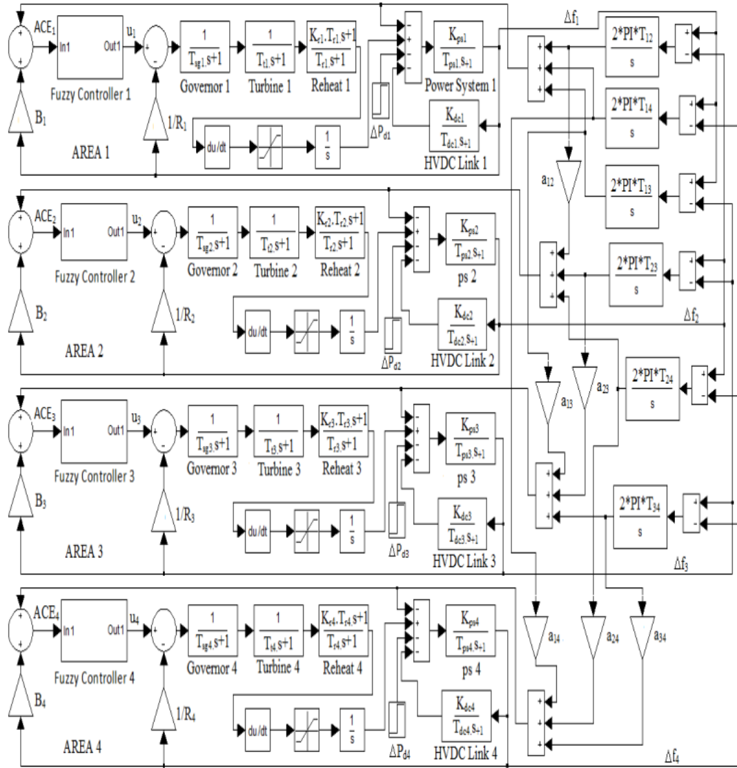
Fig 3: Transfer function model of four area interconnected power system
