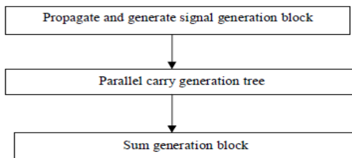
Fig 2. Addition procedure using Parallel Prefix tree structures
