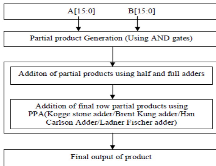
Fig.1. Block diagram of proposed Wallace tree multiplier using PPAs
