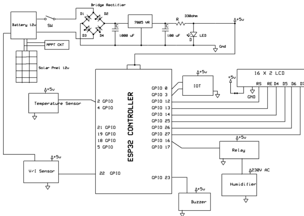
Figure 3. Circuit Diagram of Solar-Powered IoT-Based System
